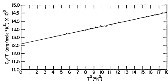
FIG. 1. A plot of C_v/T versus T^2 for NiAl between 2.2 and 4.2°K.
